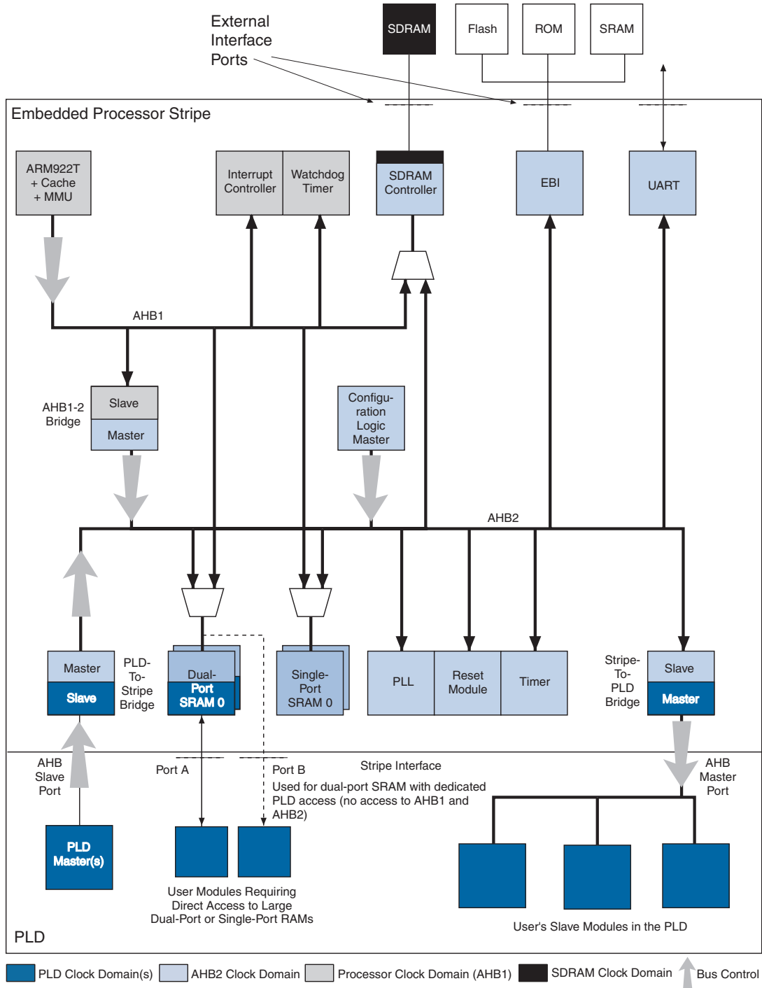
Figure 2. Excalibur System Architecture
