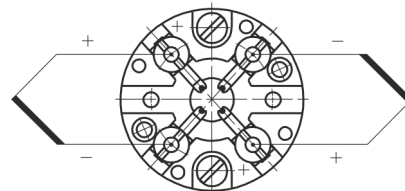
Double sensor
