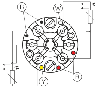
Three-wire circuit
