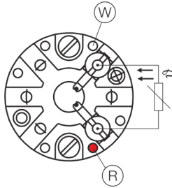
Two-wire circuit
