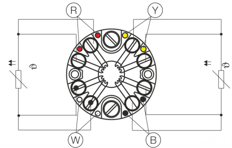
Four-wire circuit
