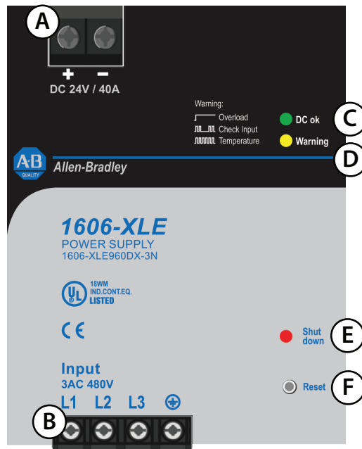
Fig. 11-1 Front side of 1606-XLE960DX-3N
