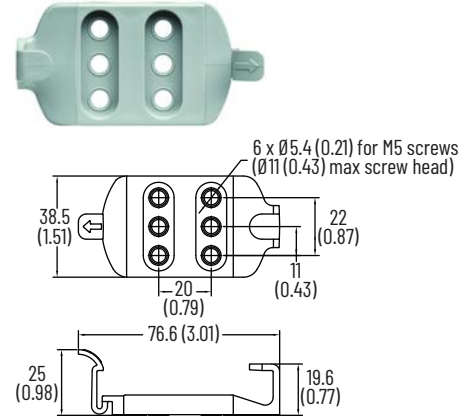
Figure 3 - 440S-GLTAPBRK1 Dimensions [mm (in.)]
